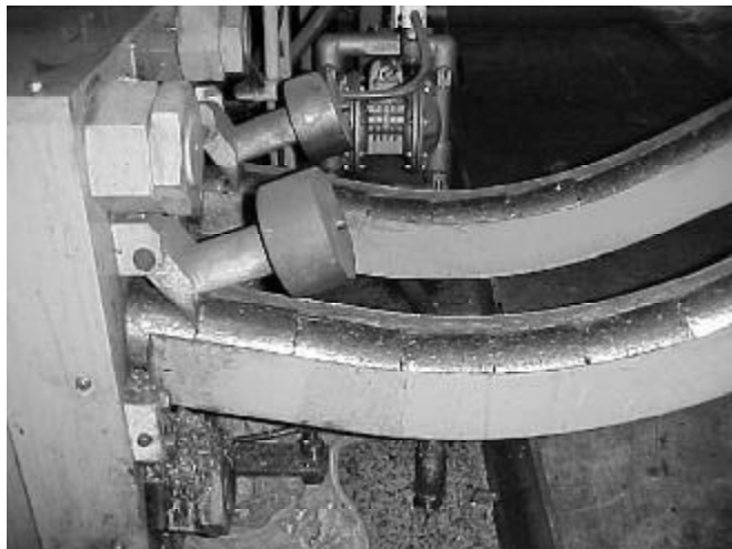
FastPac Type RB 15/3000/80 with dual discharge for aluminum briquettes.
